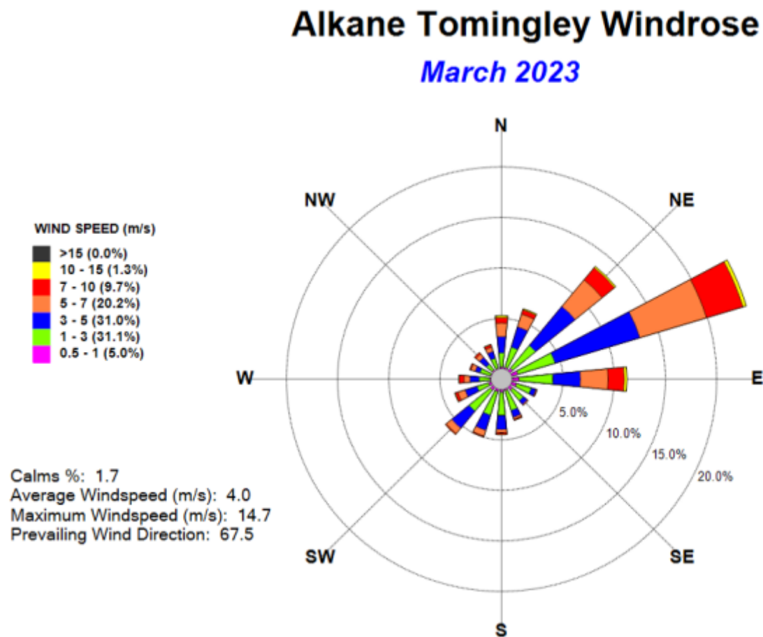
Figure 3.4: Tomingley Gold Operations Site - Windrose
