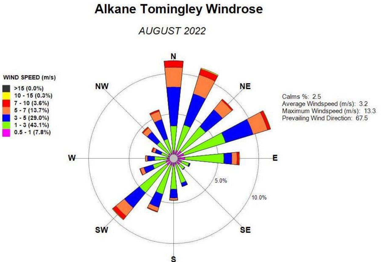
Figure 1. TGO Wind Rose
