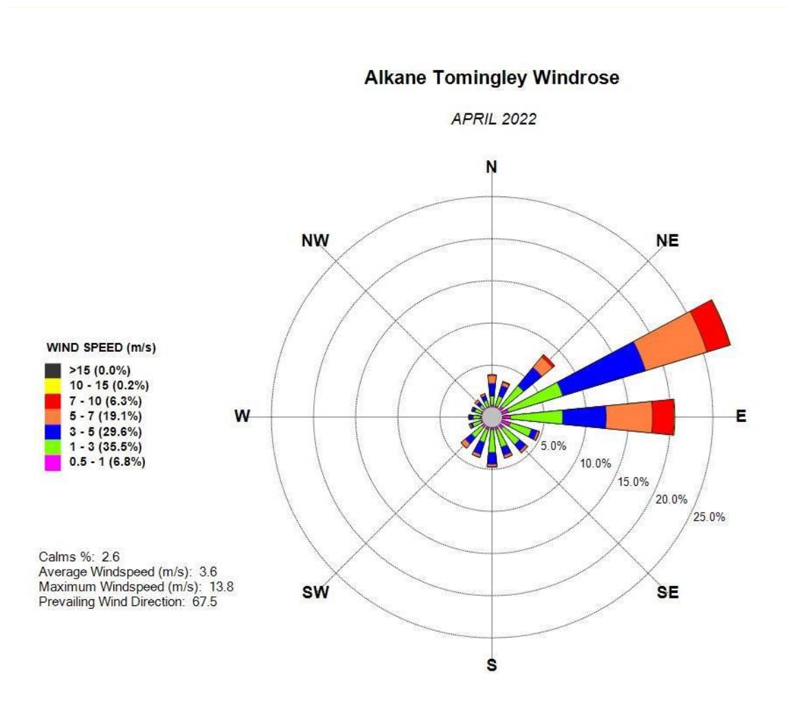
Figure 1. TGO Wind Rose
